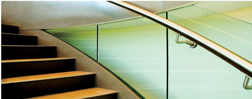
Tempered glass balustrade with stainless steel rolled 2-1/2" handrails.
